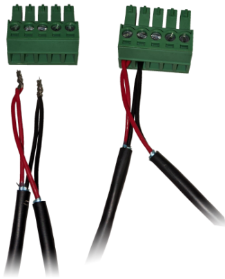
RS-485 Home-Run connection
